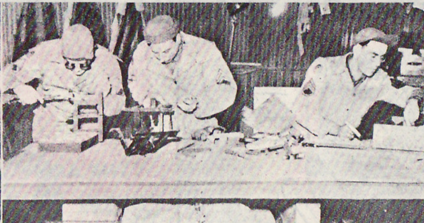
LEFT, GIs OF THE 357th FIGHTER GROUP'S SERVICE UNIT—S/SGT. OSCAR E. BRANDT OF NEHAWKA, NEB.; S/SGT. JOHN D. SCHWARZ OF WILLOW SPRINGS, MO., AND S/SGT. DAVID W. PEARCE OF NEWPORT NEWS, VA.—ARE BUSY PRODUCING GUNSIGHT MOUNTS DESIGNED BY S/SGT. IDOLO E. AUGUGLIARO OF BUFFALO, N.Y. SHOWN (RIGHT) IN A MUSTANG.
