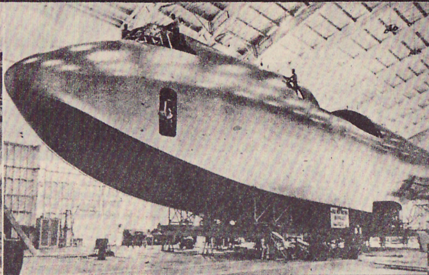
JUMBO WAIST. THIS IS THE HULL OF THE NEW "HERCULES," AND IT'S 220 FEET LONG, 30 FEET HIGH AND 25 FEET WIDE, WHICH IS EVEN LARGER THAN IT SOUNDS, IF WE'RE NOT BORING YOU. THE SHIP IS ALL WOOD, COSTS TWENTY MILLION, HAS EIGHT 3000HP ENGINES.
